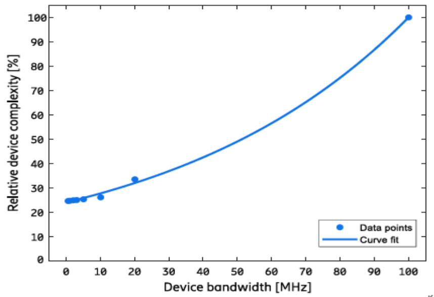
Fig 4: Relation between device complexity and device bandwidth
